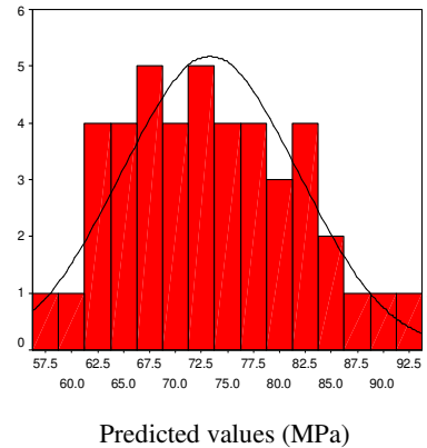
Fig. 4. Probability Curve for Experimental Values, f_{cf} .
