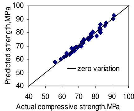
Fig. 2. Correlation of Experimental Strength with Predicted Strength, f_{cf} .
