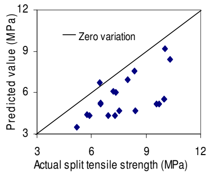
Fig. 8. Comparison of Predictions with the Experimental Results, f_{spf} of Earlier Researchers.
