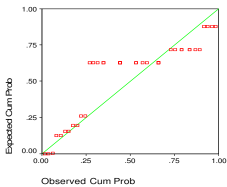
Fig. 3. Linear Probability of Predicted Compressive Strength.
