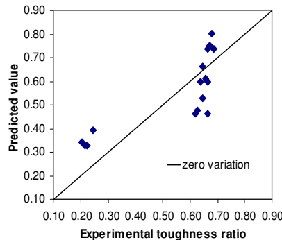
Fig. 6. Correlation of Predictions with the Experimental Results of Toughness Ratio.
