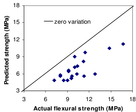
Fig. 7. Comparison of Predictions with the Experimental Results, f_{rf} of Earlier Researchers.
