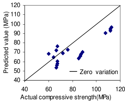
Fig. 5. Comparison of Predicted, f_{cf} with Experimental Results of Earlier Researchers.
