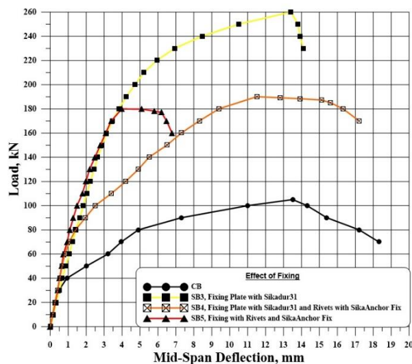
Fig. 18. Effect of the fixing of the steel plate.
