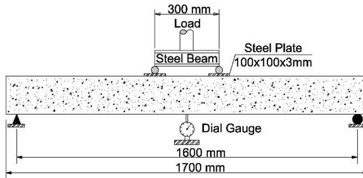
Fig. 4. Test set-up.
