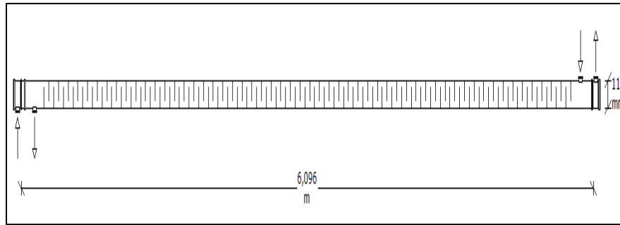
Fig. 3. Exchanger drawing.
