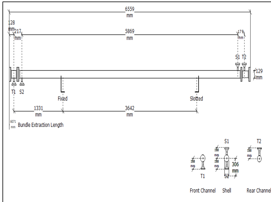
Fig. 4. Setting plan.
