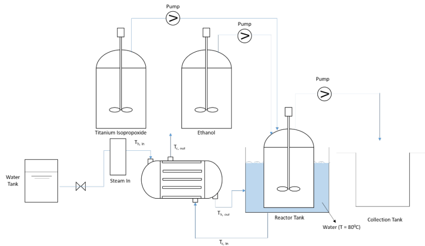
Fig. 1. Illustration of particles production.
