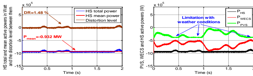
Fig. 17. Simulation results of the modified MPPT mode (with T=25^{\circ}\text{C} and g=1000\text{W/m}^2 ).
