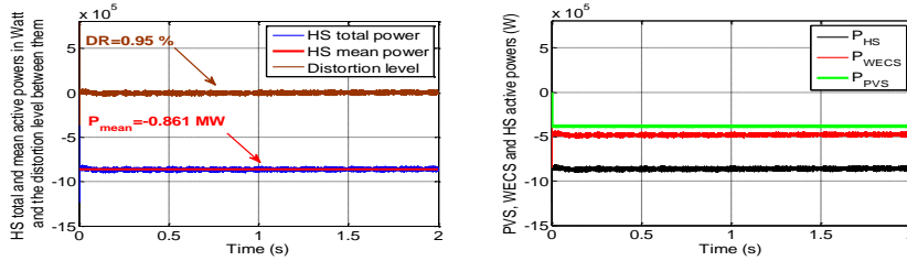
Fig. 16. Simulation results of the guaranteed minimum available power (GMAP) control mode (with T=25^{\circ}\text{C} and g=1000\text{W/m}^2 ).
