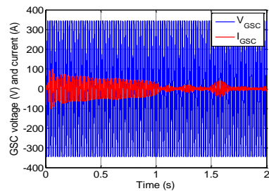
(e) GSC voltage and current.
