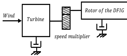
Fig. 5. Simplified mechanical model of the wind turbine.
