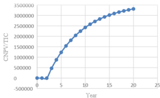
Fig. 2. Curve of ideal conditions for CNPV/TIC to a lifetime (year).
