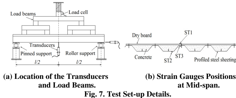
Fig. 7. Test Set-up Details.
