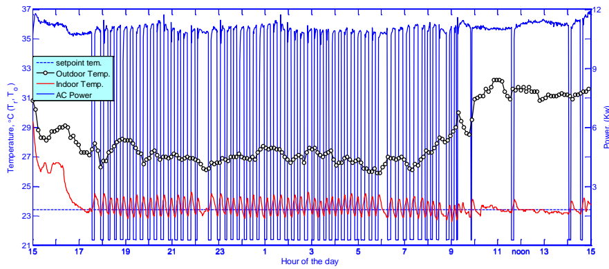
Fig. 4. Real temperature and power consumption for AC load.
