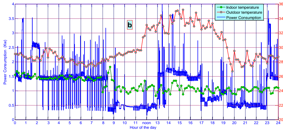
(b) Weekend power consumption pattern.
