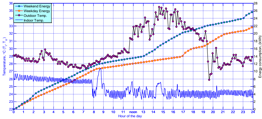
Fig.3. Energy consumption pattern of households with outdoor and indoor temperature during weekdays and weekends.
