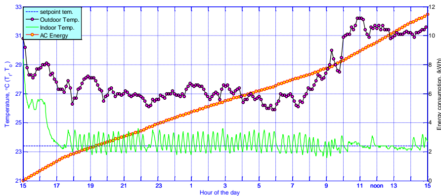
Fig. 5. Energy consumption of AC with outdoor and indoor temperature.
