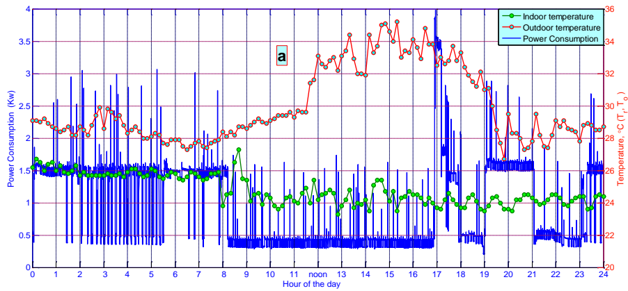
(a) Weekday power consumption pattern.
