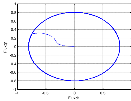
Fig. 13. Motor1 Flux Circle Curve.
