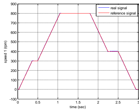
Fig. 17. Reference speed and rotation speed of motor1.
