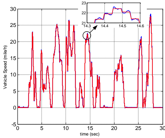
Fig. 7. Vehicle speed curve with NYCCDS driving cycle.
