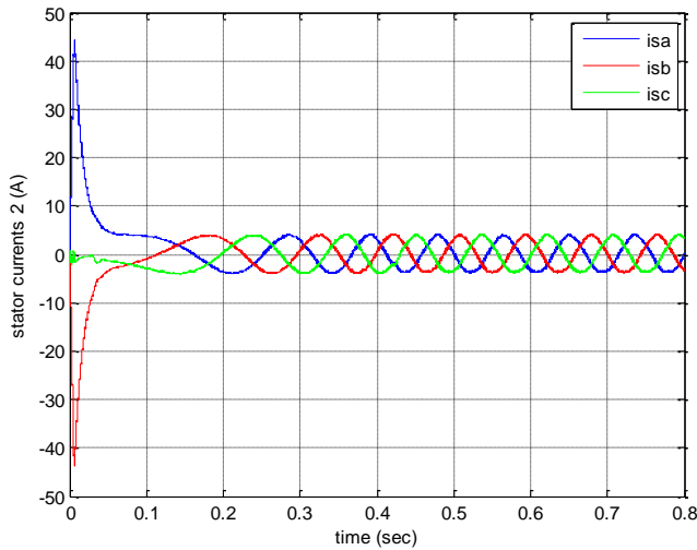
Fig. 16. Motor2 Three-Phase Current.
