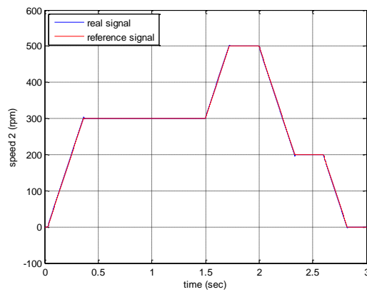
Fig. 18. Reference speed and rotation speed of motor2.
