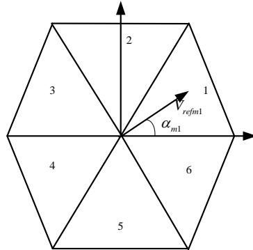
Fig. 4. Space vector classification.
