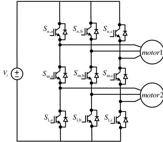
Fig. 1. Nine-switch inverter structure.
