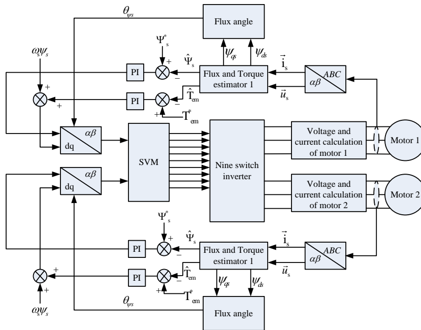
Fig. 2. Proposed SVM-DTC control diagram.
