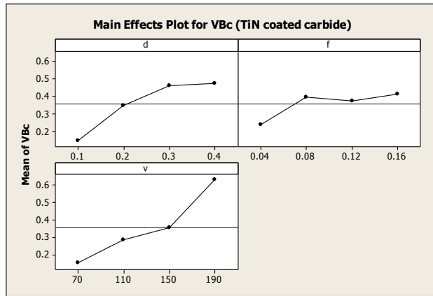
Fig. 5. Main effects plot for VBc .
