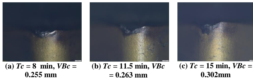
Fig. 4. Images of flank wear with successive machining time at run 1 ( d = 0.1 mm, f = 0.04 mm/rev and v = 70 m/min).
